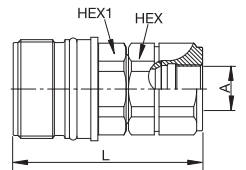
Female BSPP Thread – DIN 3852 Form Y
