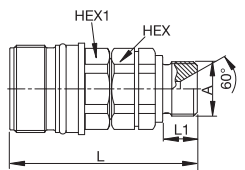
Male BSPP Thread – DIN 3852 Form B
