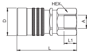
Female Thread
