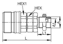
Male Thread 24° cone – DIN 2353 Bulkhead
